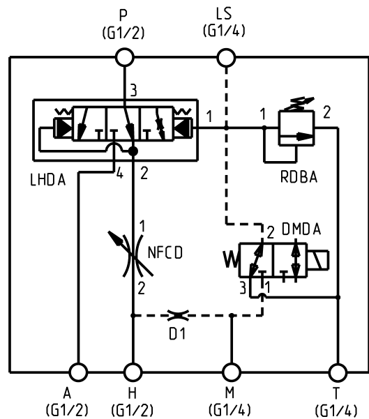
SCHEMA: A310-01D-G01
