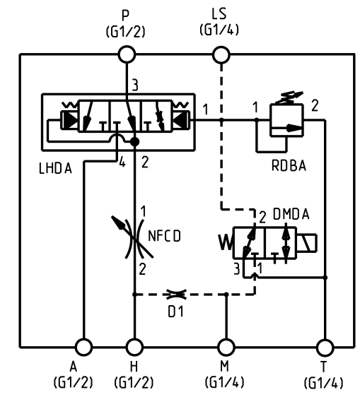
SCHEMA: A310-01D-G01
