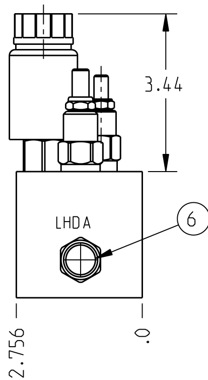
SCHEMA: A310-01D-G01
