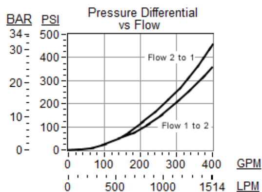
Model LOKB installed in T-19AU Cavity
