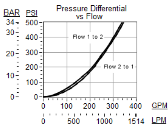
Model LOKB installed in T-19A Cavity
