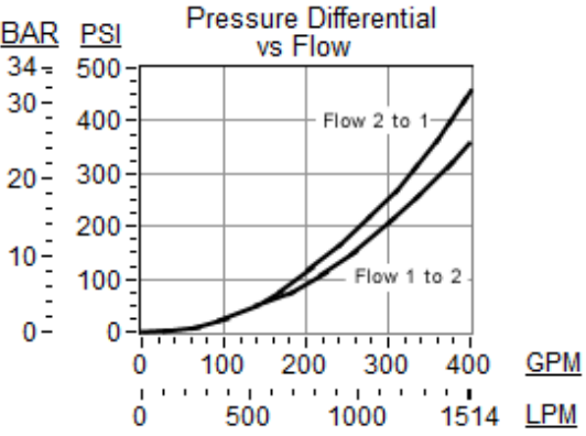
Model LOKB8 installed in T-19AU Cavity
