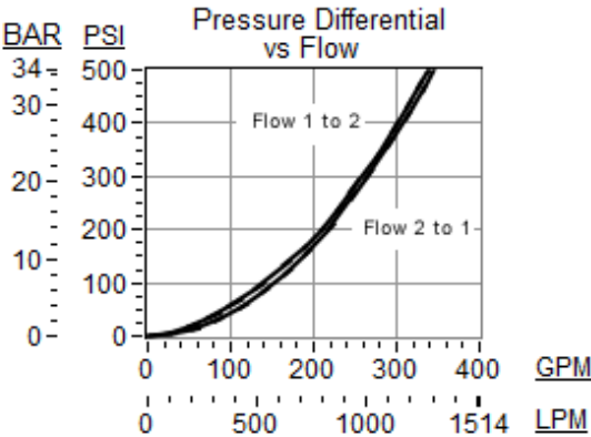
Model LOKD8 installed in T-19A Cavity
