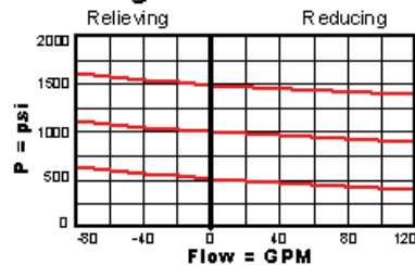
Regulated Pressure
