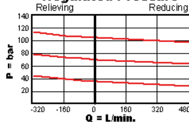
Regulated Pressure
