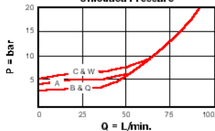
Unloaded Pressure
