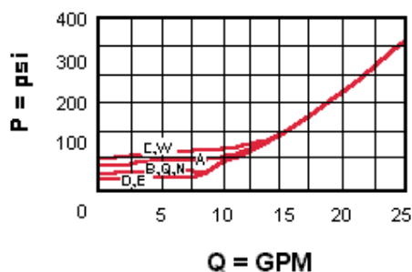
Unloaded Pressure
